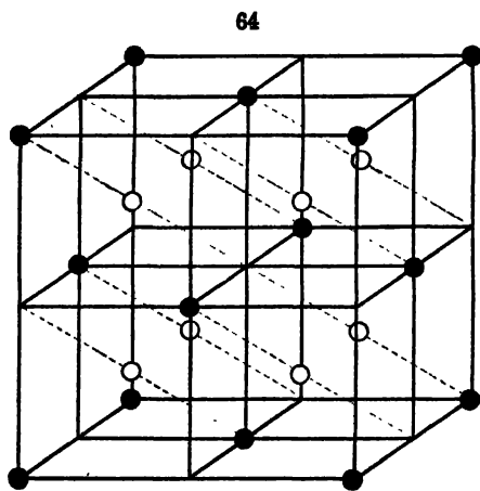
Structure of Fluorite: Ca = ●, F = ○
